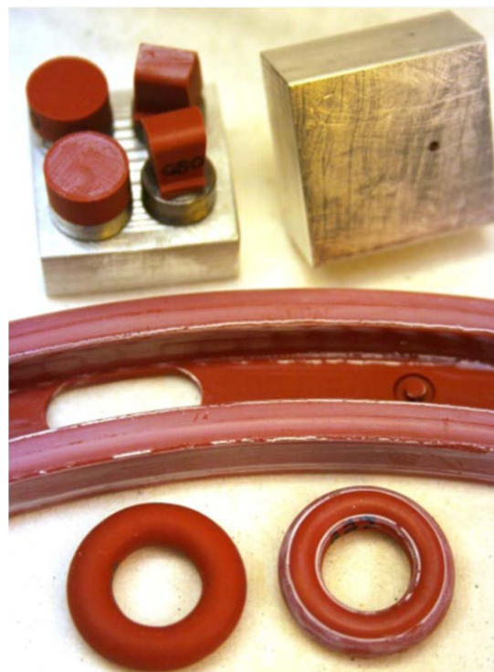
Figure 2. Adhesion specimens and 1 inch square vented block used with #2-309 O-rings. Top left: buttons and cut sections of Medium-scale seals (Mss) after adhesion testing. Center: Medium-scale seal after coating and adhesion testing. Bottom: #2-309 O-rings.
