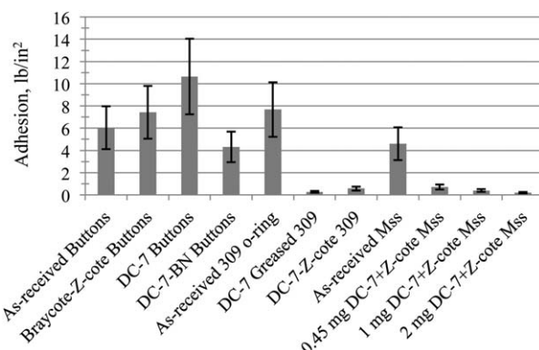
Figure 3. Average adhesion of buttons, 2-309 O-rings coated with 0 or 2 mg/cm 2 , and cut sections from Medium-scale seals (Mss) coated with 0, 0.45, 1, and 2 mg/cm 2 ; 1 lb/inch 2 = 6.9 kPa.
