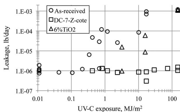
Figure 6. Small-scale seal leakage after UV-C exposure, as-received, coated with 2 \text{ mg/cm}^2 DC-7-16.4%Z-cote sunscreen, and with 6% TiO 2 added to the compound; 1 \text{ lb/day} = 0.454 \text{ kg/day} .
