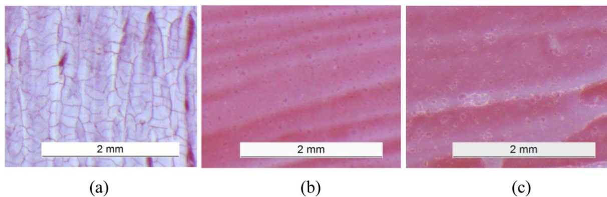
Figure 5. Optical images of small-scale seals: (a) coated with Braycote-20%Z-cote and exposed to 1 \times 10^{20} atoms/cm 2 AO; (b) coated with DC-7-16.4%Z-cote prior to AO exposure; (c) coated with DC-7-16.4%Z-cote and exposed to 4.6 \times 10^{20} atoms/cm 2 AO.
