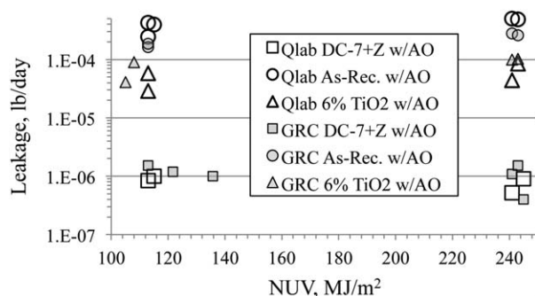
Figure 7. Leakage, after NUV + AO exposure, of small-scale seals as-received, coated with 2 mg/cm 2 DC-7–16.4%Z-cote sunscreen, and with 6% TiO 2 added to the compound prior to curing; 1 lb/day = 0.454 kg/day.
