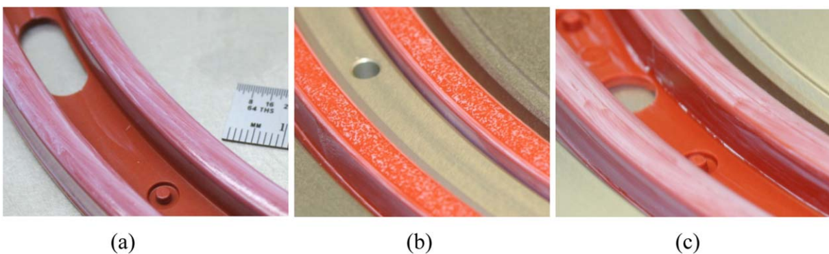
Figure 10. (a) Medium-scale seal -0282 after coating; (b) Coated -0282 after adhesion testing at -50^\circ\text{C} ; (c) Coated Medium-scale seal -0283 after adhesion testing at -8^\circ\text{C} .
