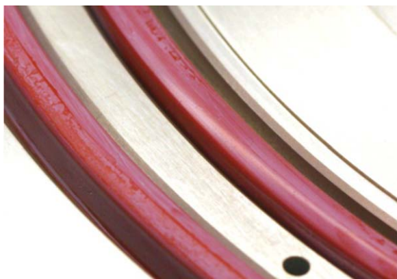
Figure 11. Coated medium-scale seal -0283 after adhesion testing at -8^{\circ}\text{C} (8 h, dwell) and then 25 more times at room temperature (1 min dwell on each cycle).
